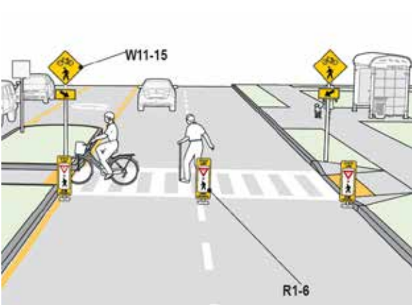
Figure 70. In-Street Path Crossing (AASHTO)
