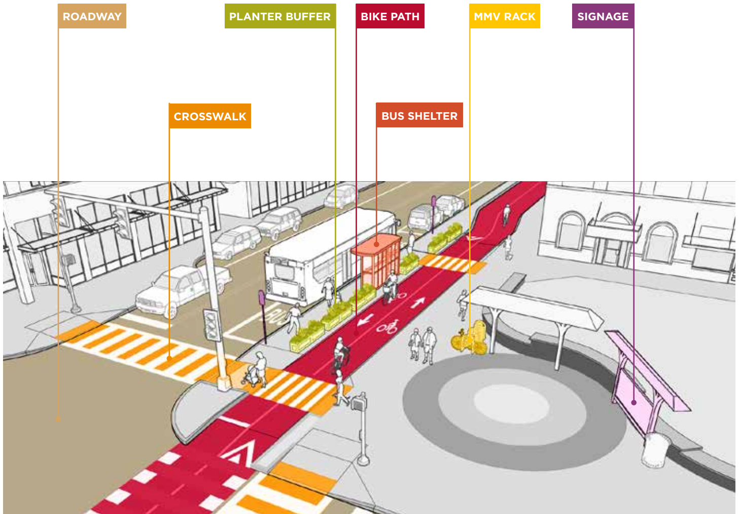
Figure 110. Floating Bus Stop, 2024 AASHTO Bike Guide
