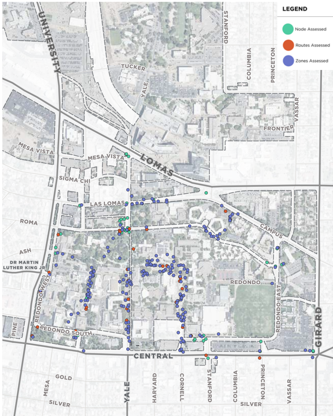
Map 21. Features Assessed
