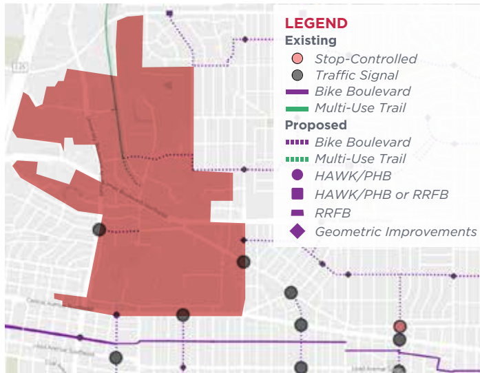
Map 4. Enhanced Crossings
