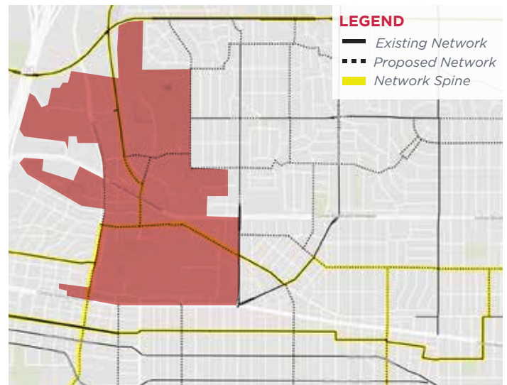
Map 5. Network Spines
